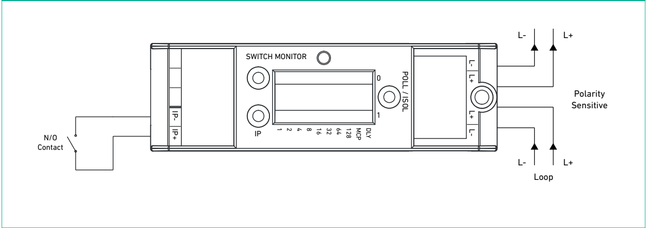
Figure 3: Intelligent Twin Switch Monitor normally open monitoring mode connectivity diagram (compatible with CoreProtocol only)
