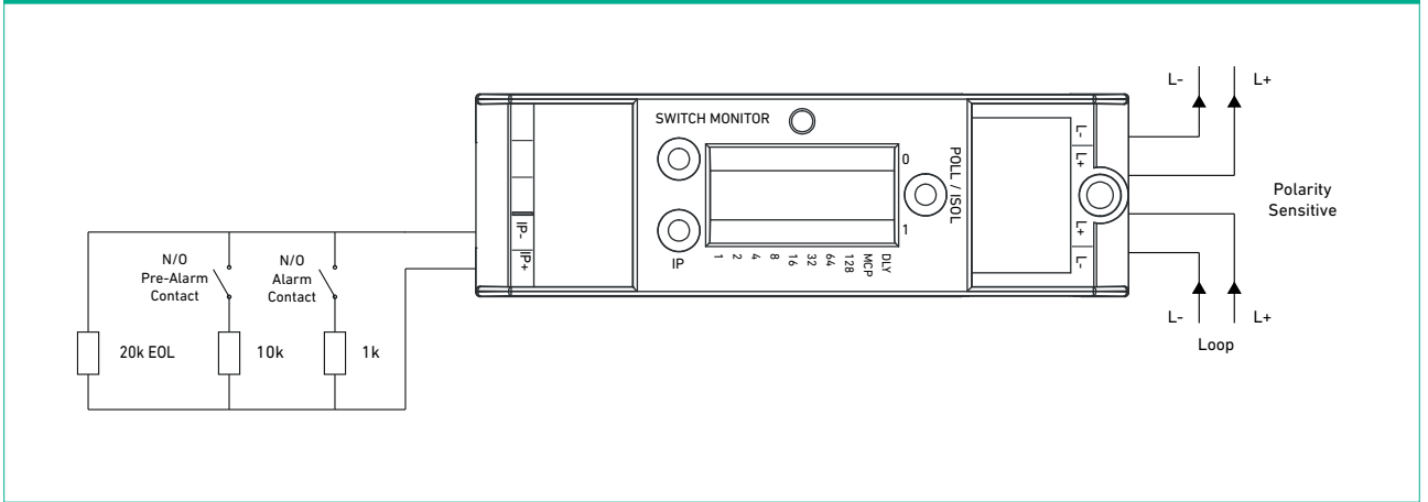
Figure 2: Intelligent Twin Switch Monitor standard resistive monitoring mode connectivity diagram
