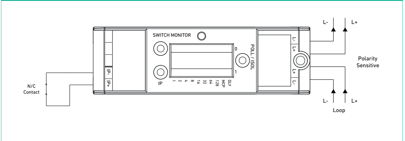
Figure 4: Intelligent Twin Switch Monitor normally closed monitoring mode connectivity diagram (compatible with CoreProtocol only)
