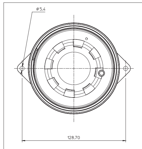
Figure 1: Fixing hole centres
